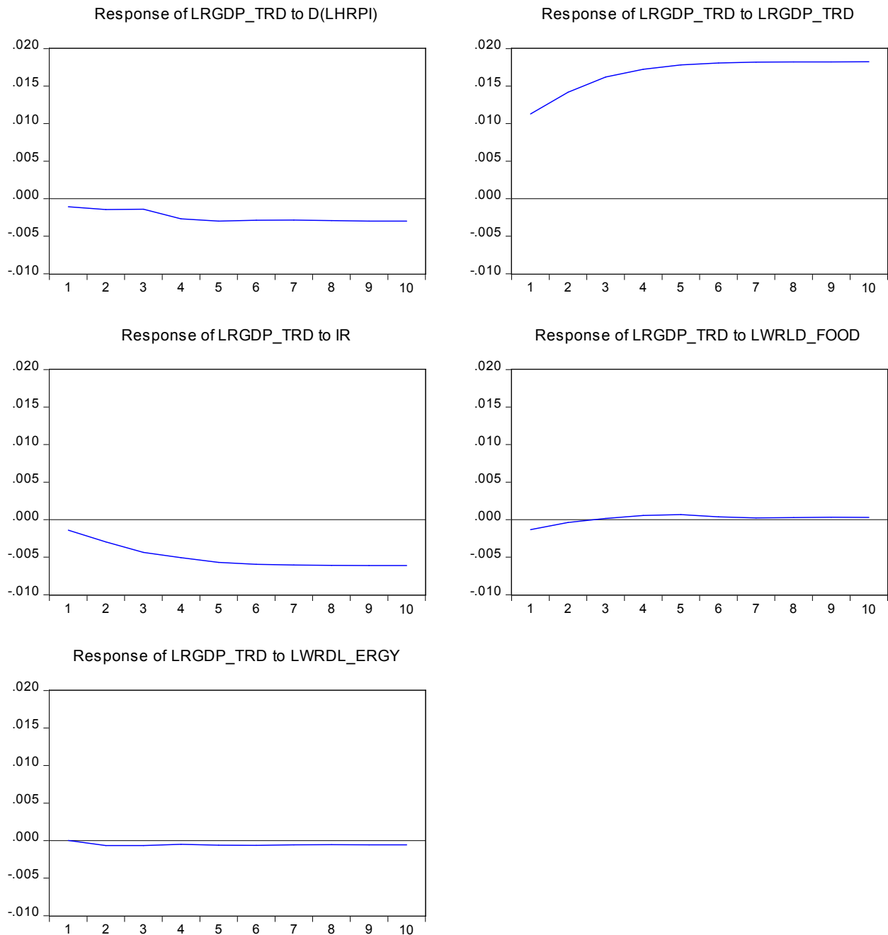
Figure 41: Impulse Responses of LRGDP to Generalised 1 S.D. Innovations
